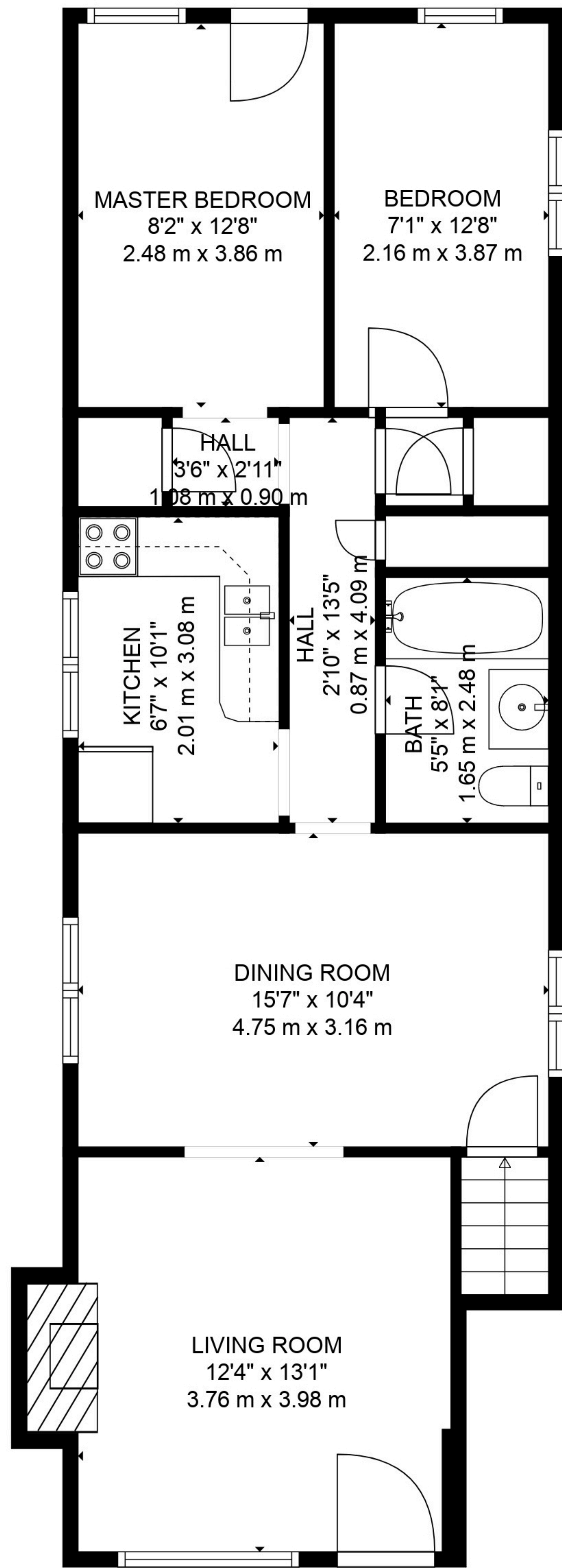
MAIN FLOOR
