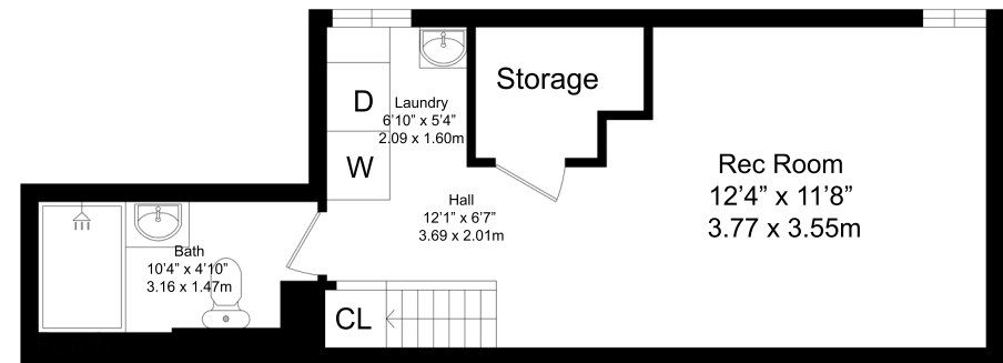
BASEMENT 337 ft 2
