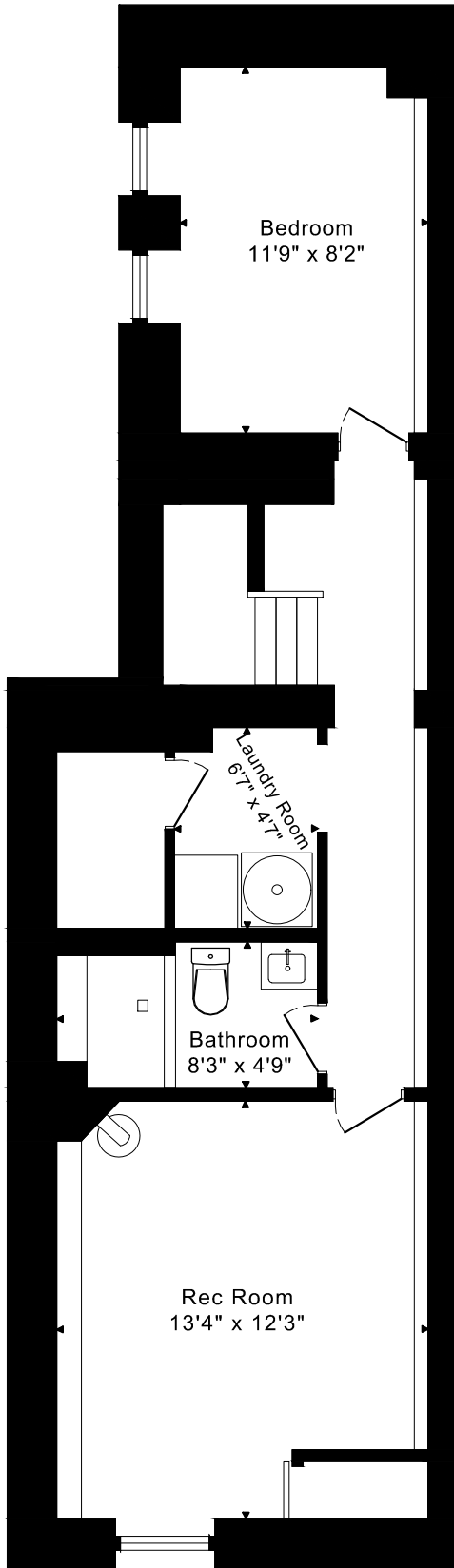
LOWER FLOOR 650 SQUARE FEET
