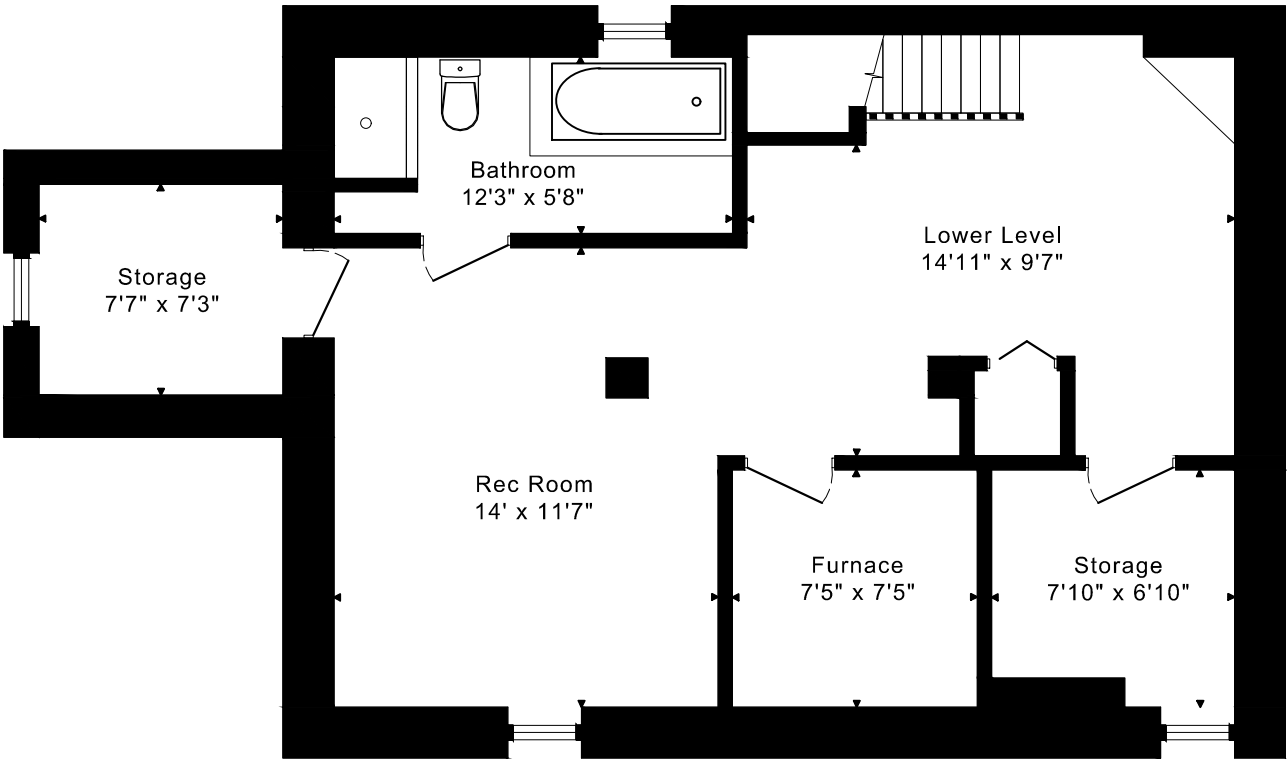
LOWER FLOOR 810 SQUARE FEET
