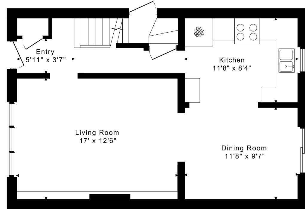
MAIN FLOOR 635 SQUARE FEET
