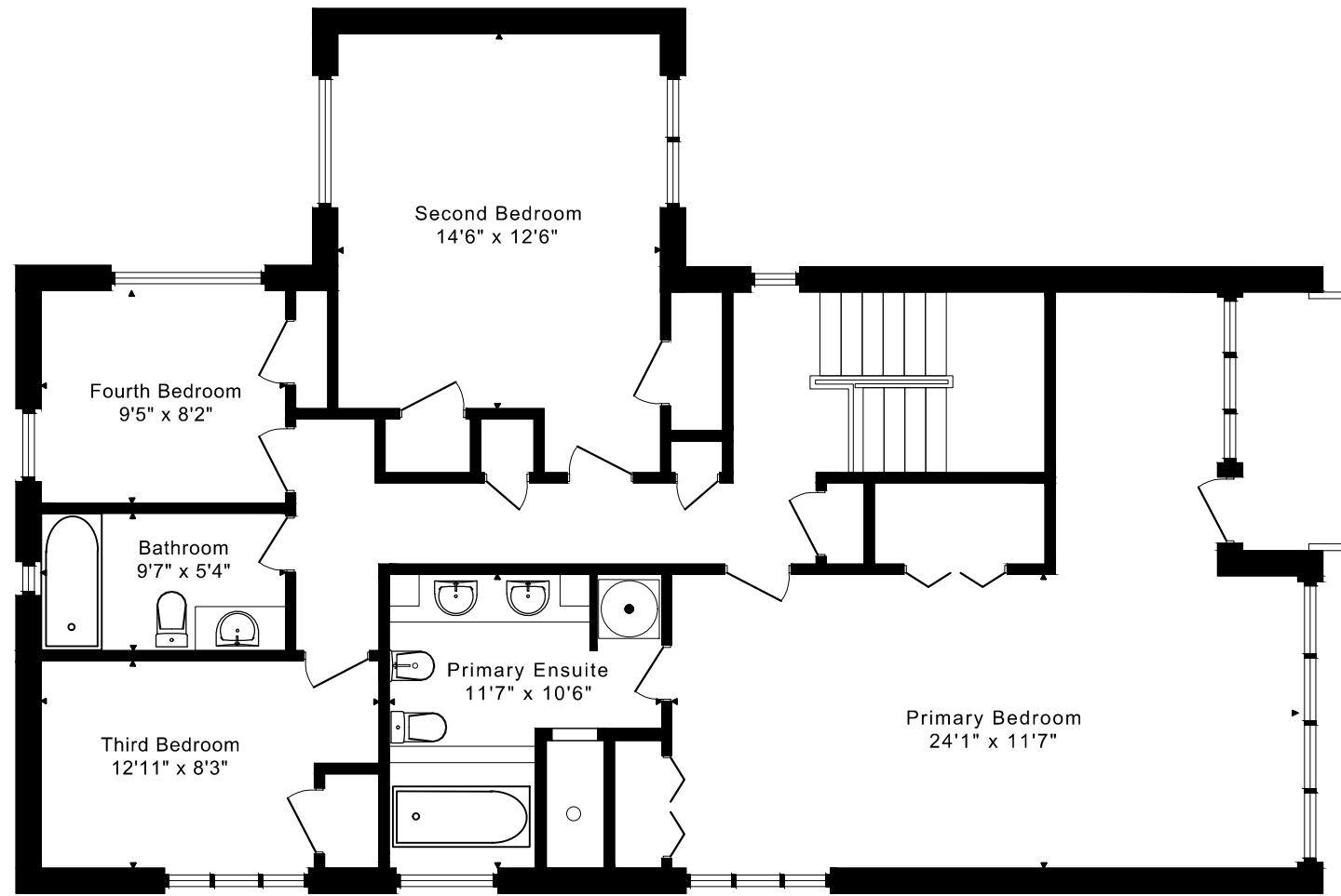
SECOND FLOOR 1390 SQUARE FEET
