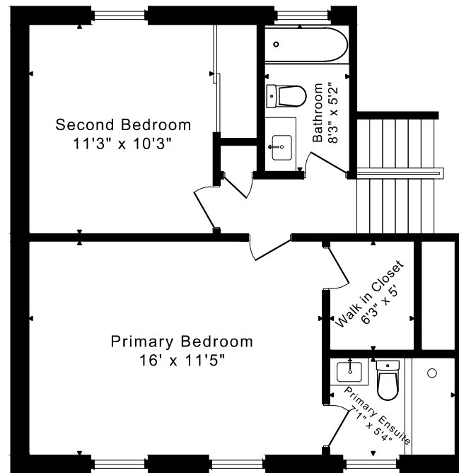
SECOND FLOOR 580 SQUARE FEET
