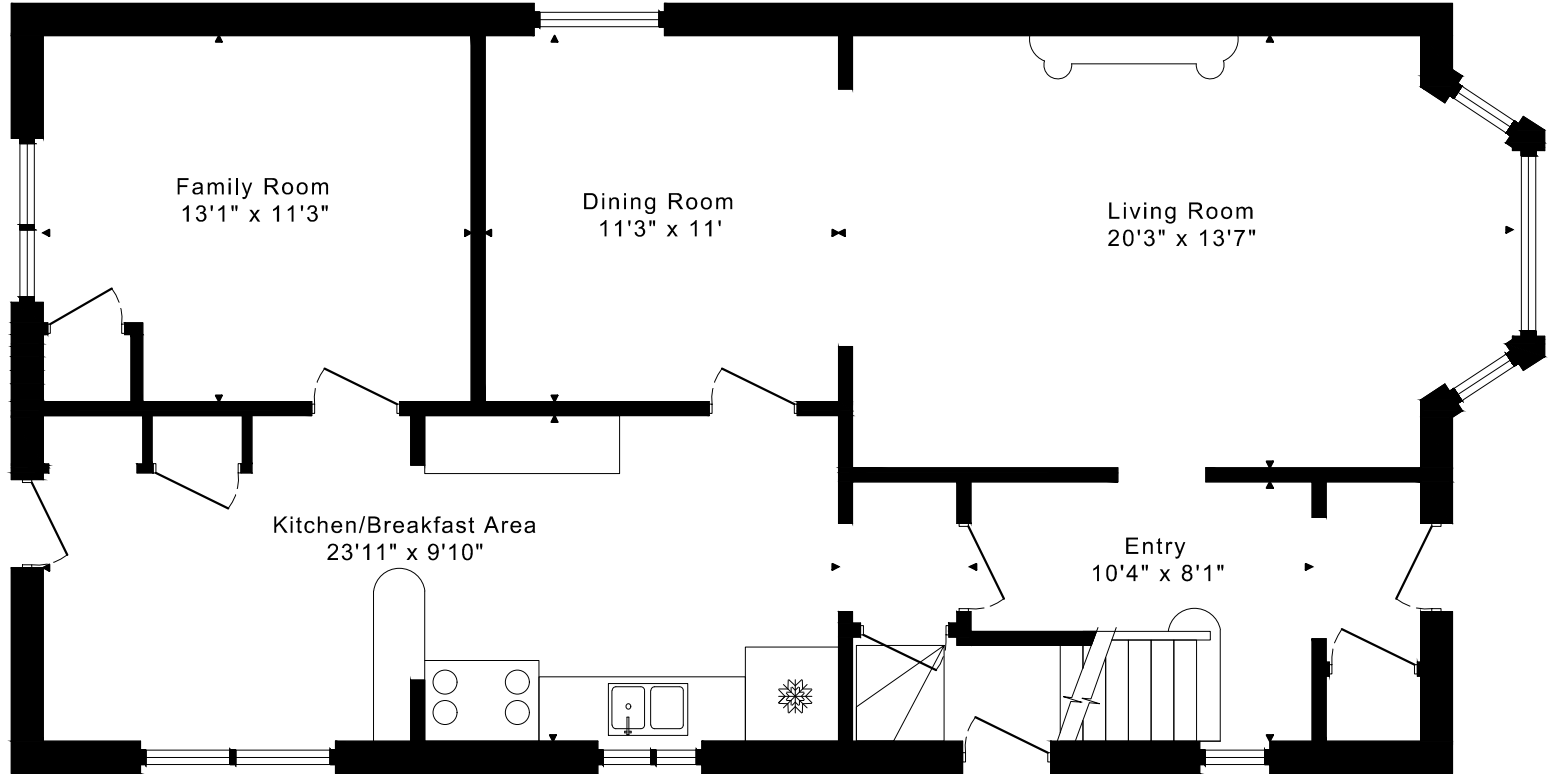
MAIN FLOOR 1070 SQUARE FEET
