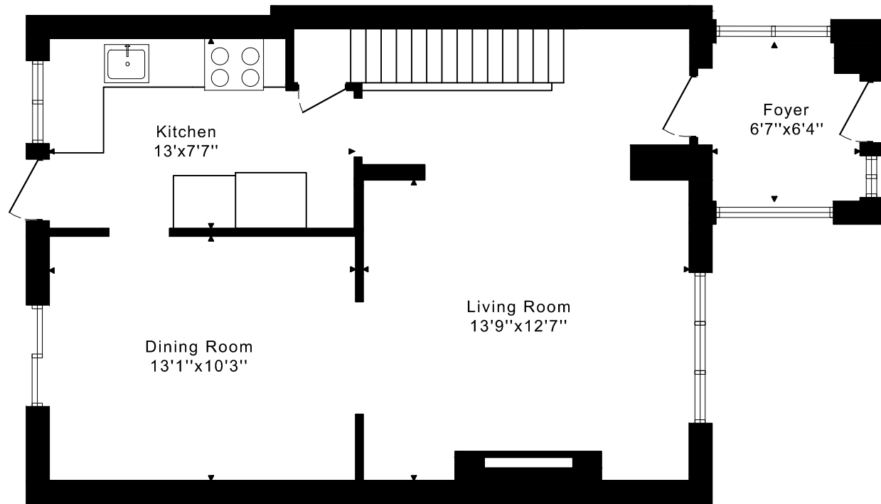
MAIN FLOOR 695 SQUARE FEET
