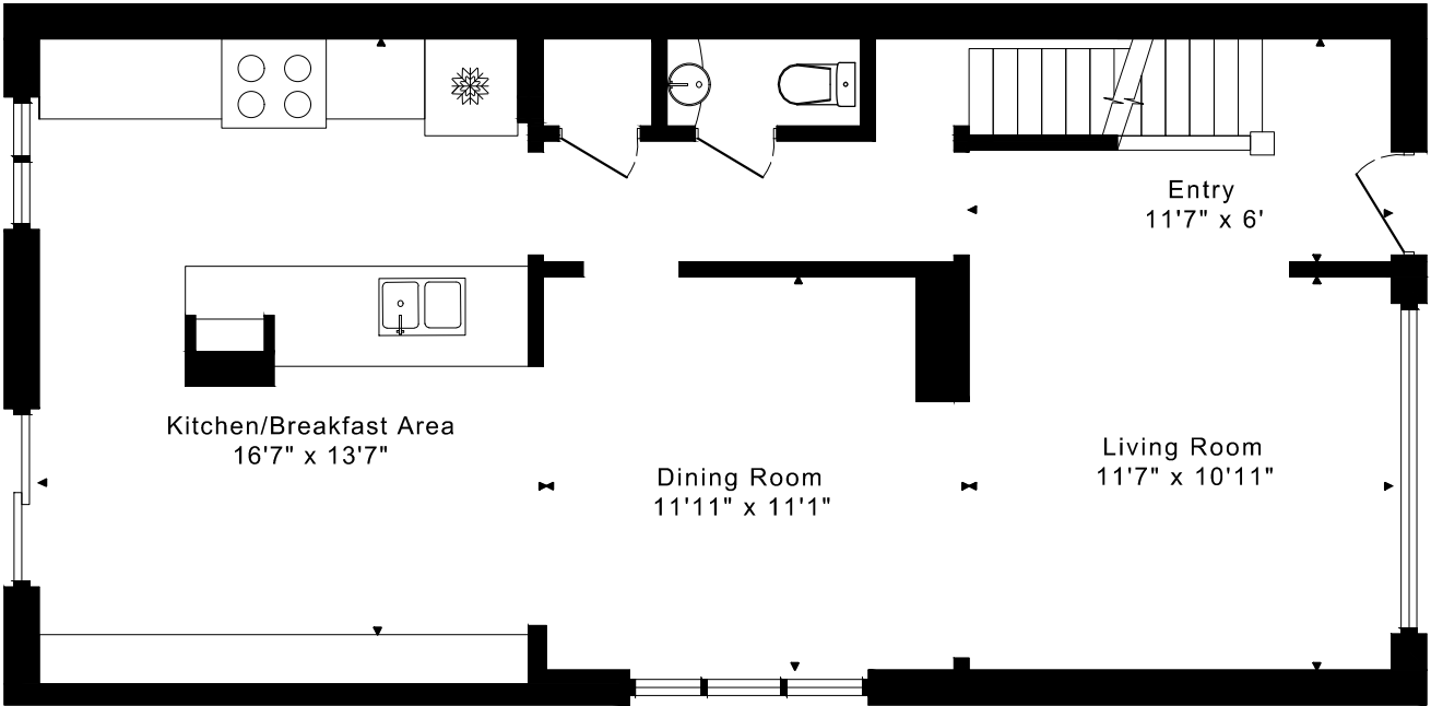
MAIN FLOOR 780 SQUARE FEET
