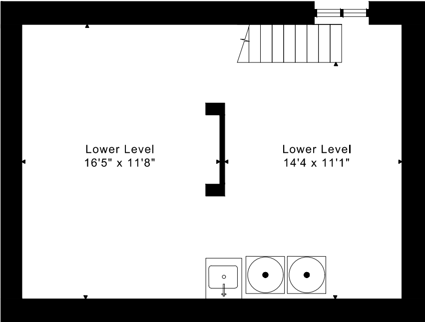
LOWER FLOOR 510 SQUARE FEET
