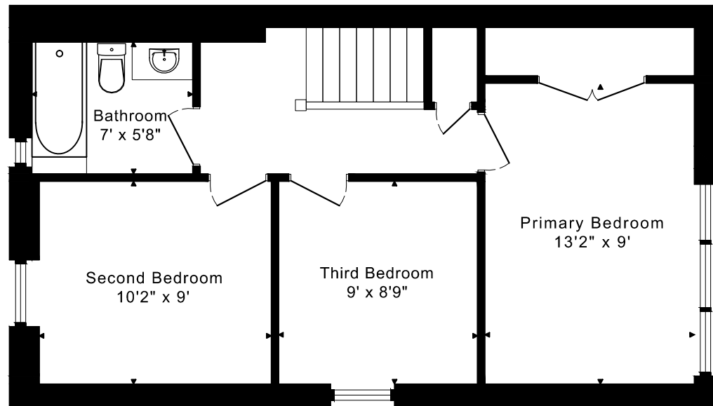
SECOND FLOOR 540 SQUARE FEET
