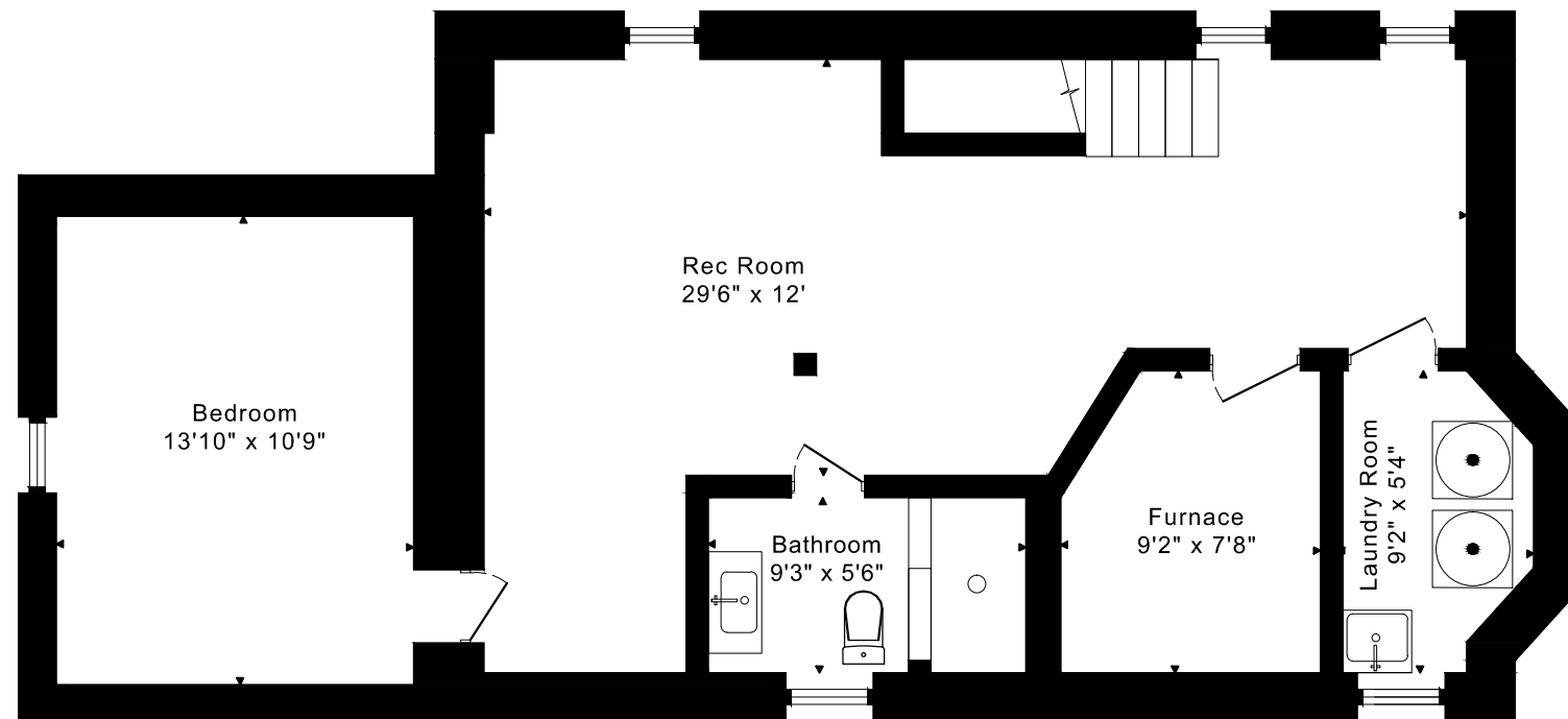
LOWER FLOOR 885 SQUARE FEET
