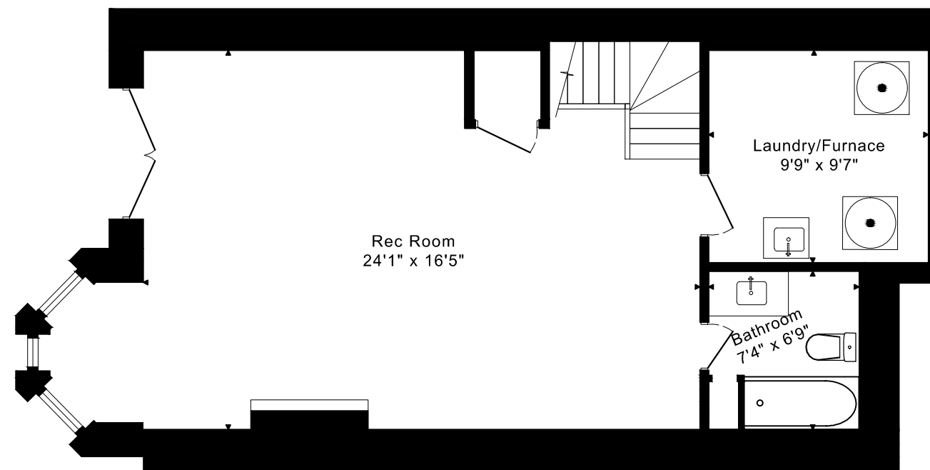
LOWER FLOOR 735 SQUARE FEET
