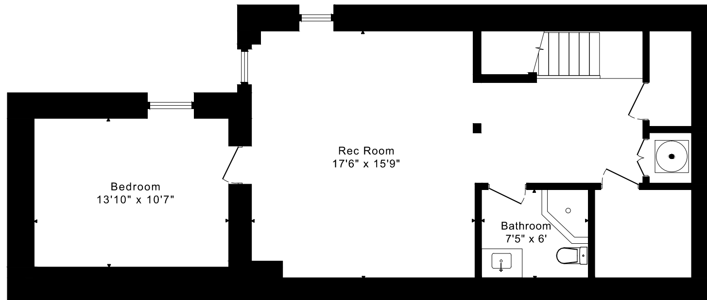
LOWER FLOOR 950 SQUARE FEET
