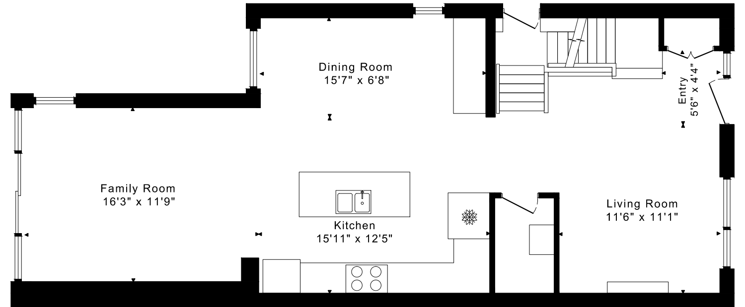
MAIN FLOOR 950 SQUARE FEET
