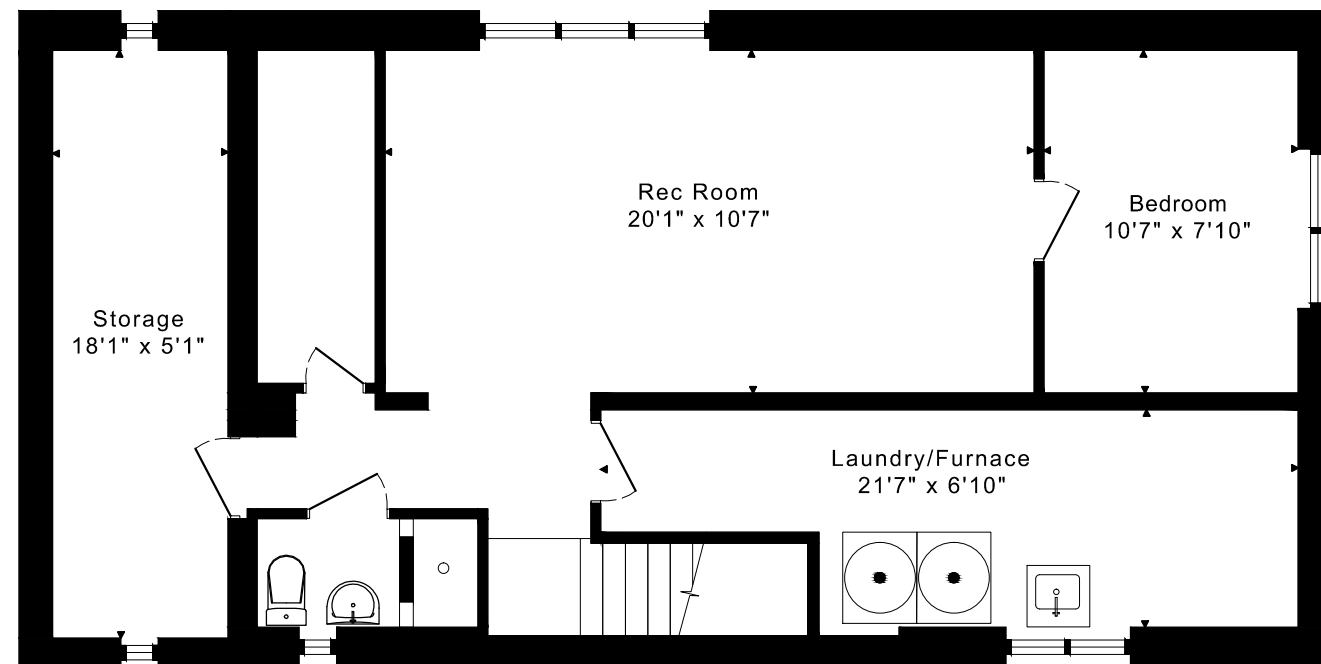
LOWER FLOOR 825 SQUARE FEET
