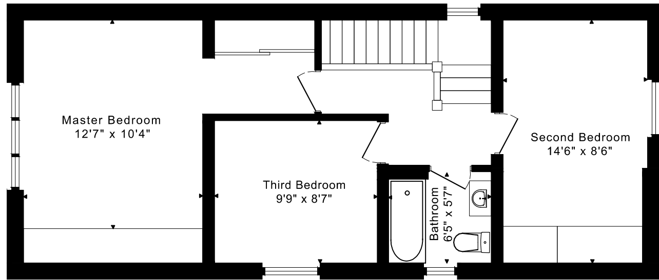
SECOND FLOOR 655 SQUARE FEET
